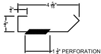
PERFORATED CHANNEL
